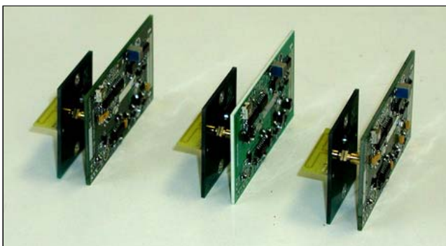
Three prototypes of the GuardDog Ultra-Wideband Intrusion Detector for MachineTalker attachment
